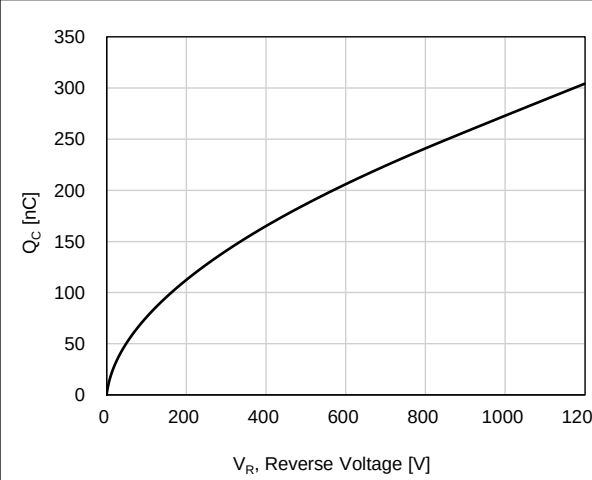
Figure 5. Capacitive Charge Characteristics
