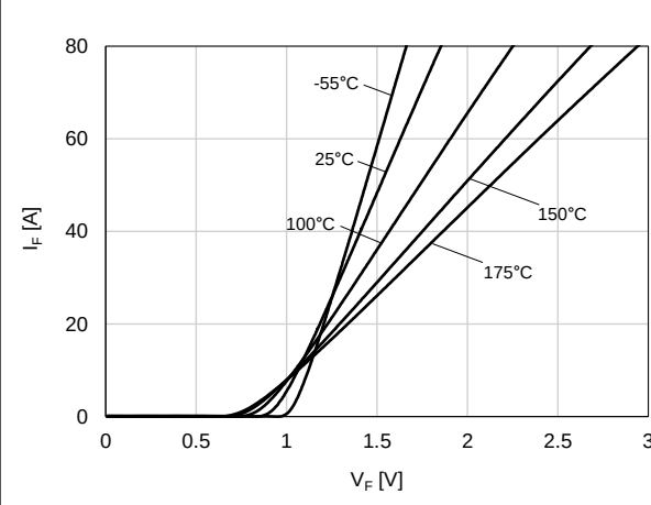
Figure 3. Forward Characteristics
