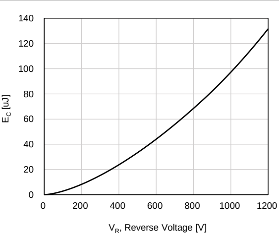
Figure 6. Capacitance Stored Energy
