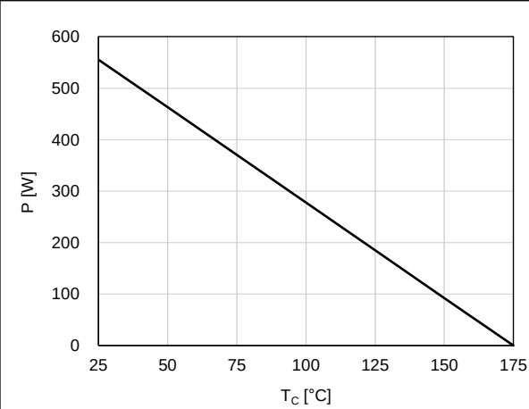
Figure 1. Power Derating
