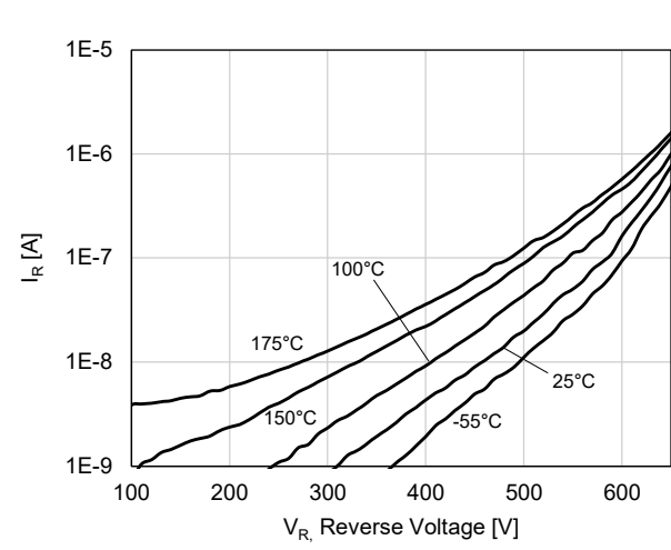
Figure 4. Reverse Characteristics
