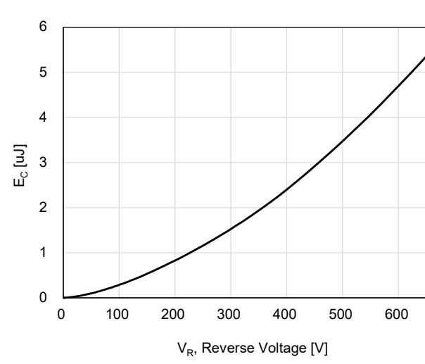
Figure 6. Capacitance Stored Energy
