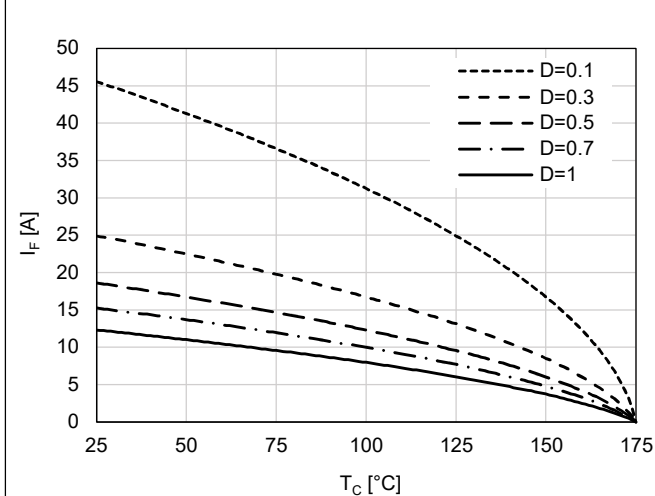
Figure 2. Current Derating
