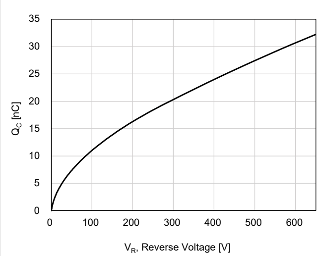
Figure 5. Capacitive Charge Characteristic
