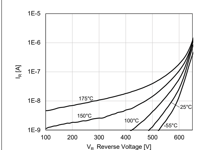
Figure 4. Reverse Characteristics
