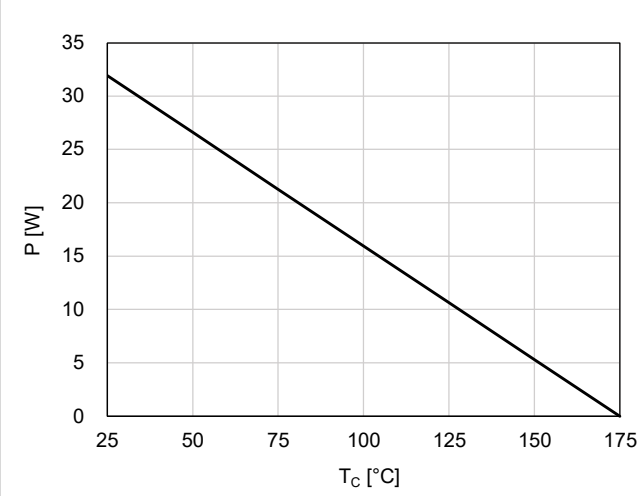
Figure 1. Power Derating
