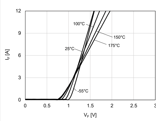
Figure 3. Forward Characteristics
