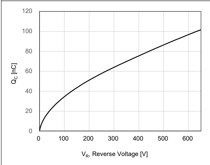
Figure 5. Capacitive Charge Characteristic
