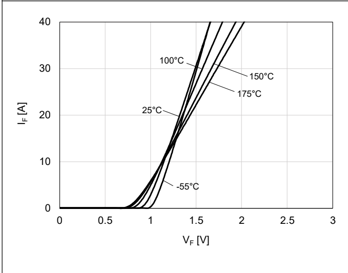
Figure 3. Forward Characteristics
