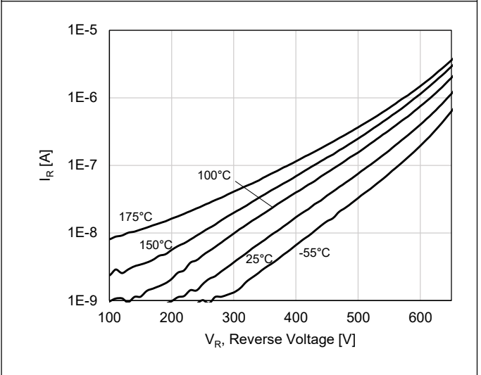
Figure 4. Reverse Characteristics
