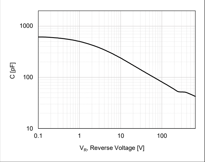
Figure 7. Capacitance Characteristic
