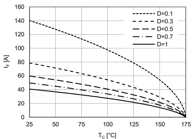
Figure 2. Current Derating
