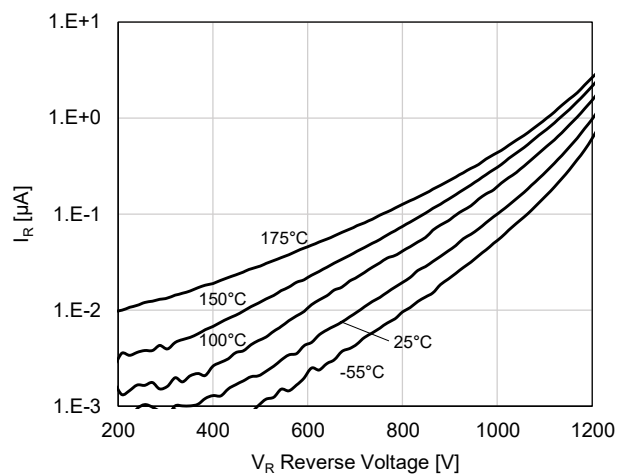
Figure 4. Reverse Characteristics
