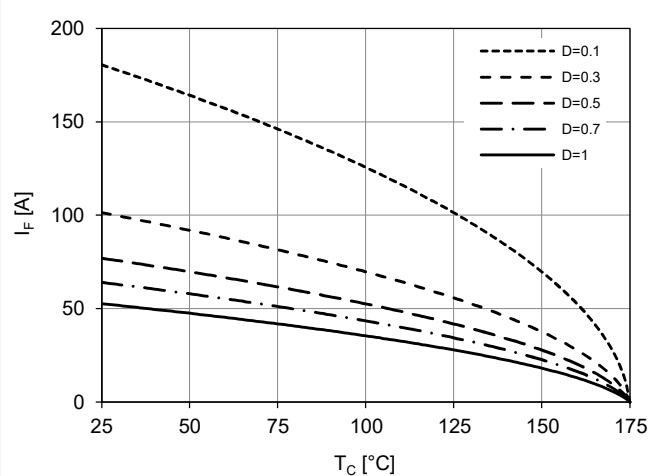
Figure 2. Current Derating
